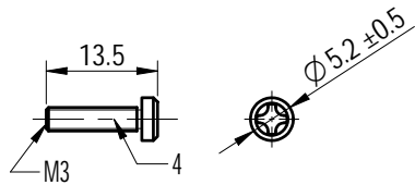
SCREW-1
