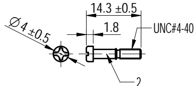
Short BOLT
