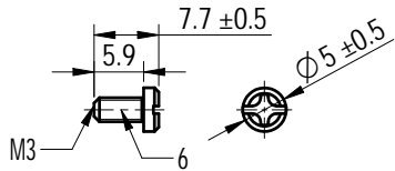
SCREW-2
