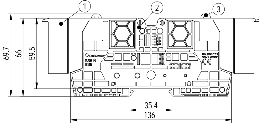
面板安装示意图/Panel installation diagram
