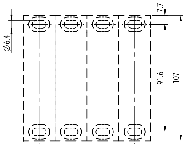
面板安装示意图/Panel installation diagram
