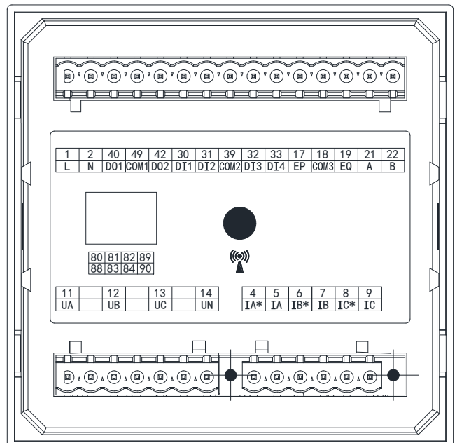
Figure 18 DEMP-AC3-D92 Extended WF/LoRa Wiring Diagram
