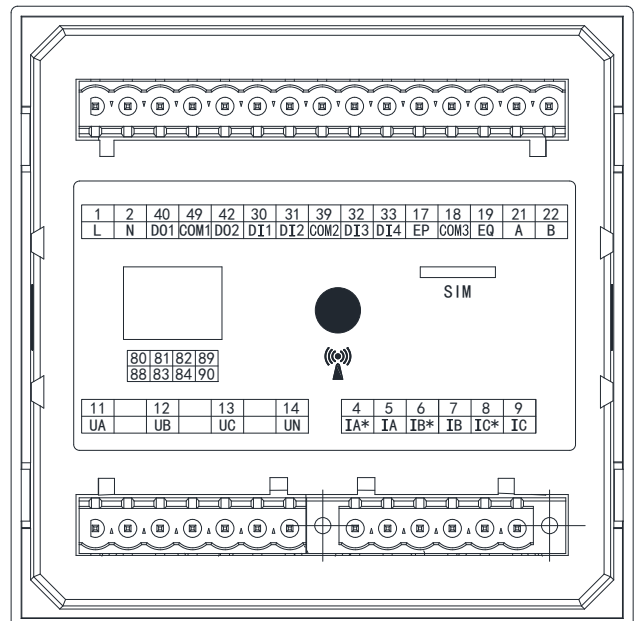
Figure 16 DEMPSeries AC3-D92 Extended 4G Wiring Diagram
