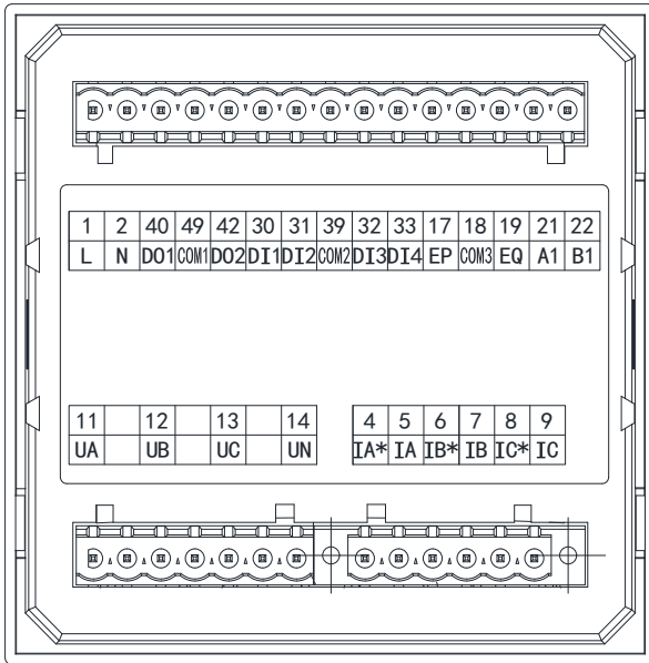
Figure 13 DEMPSeries AC3-D92 basic wiring diagram
