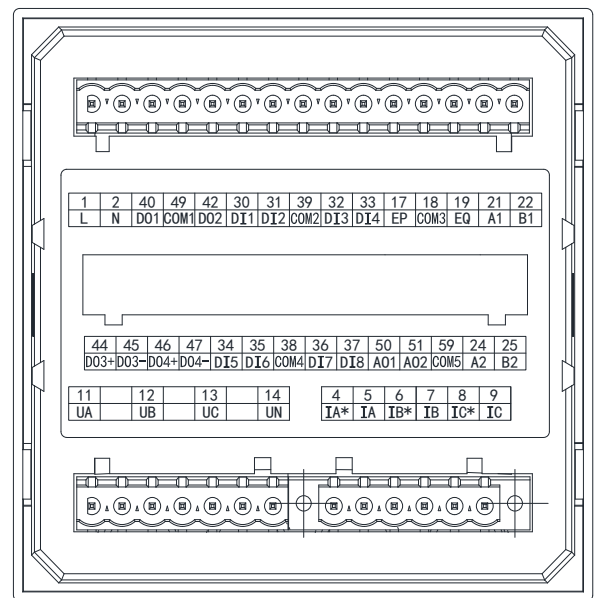
Figure 14 DEMPSeries AC3-D92 extended K/2M/2C wiring diagram
