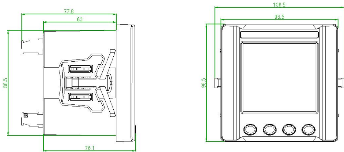
Figure 3 DEMPSeries AC3-D92 dimensional drawing
