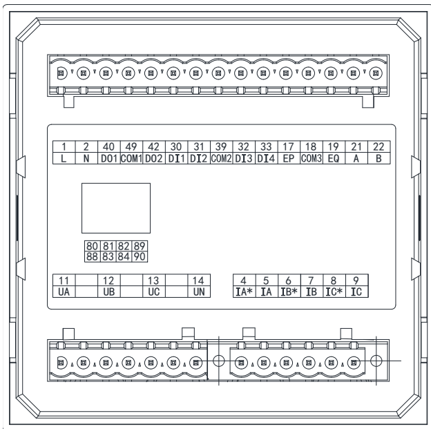
Figure 15 DEMPSeries AC3-D92 Extended Ethernet/Temperature Measurement/Leakage Wiring Diagram
