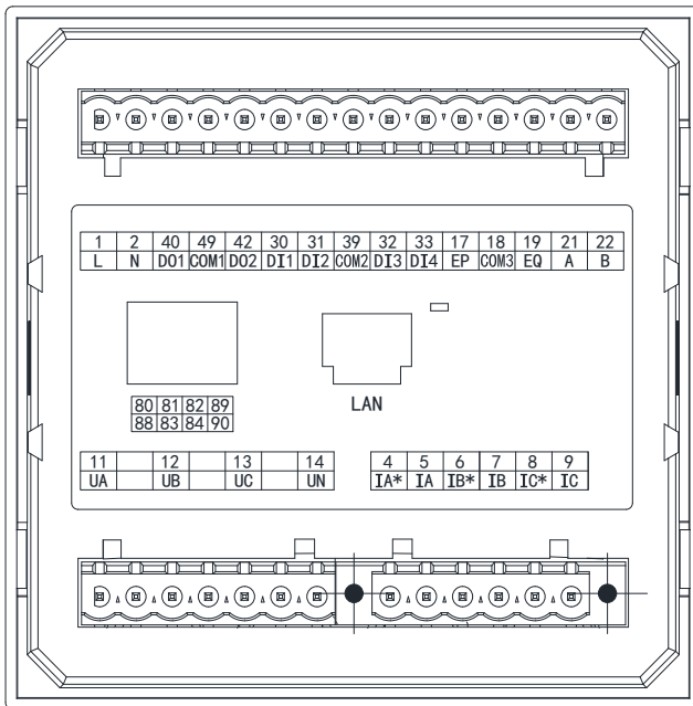
Figure 17 DEMP-AC3-D92 Extended CE Wiring Diagram
